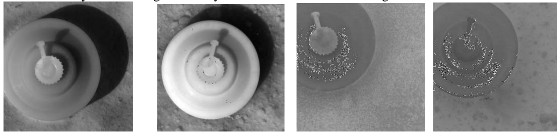
Surface mine
