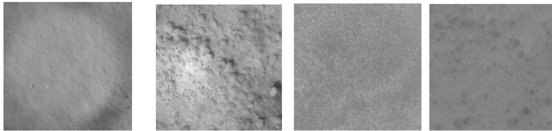
Flush-buried mine
